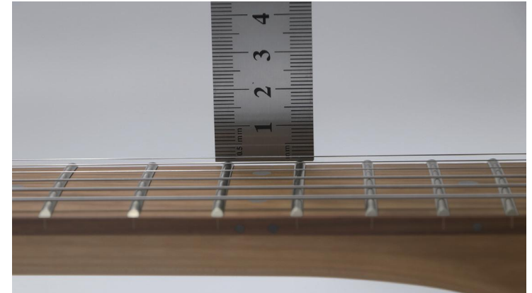
Bass side (6th string) at the 12th fret
