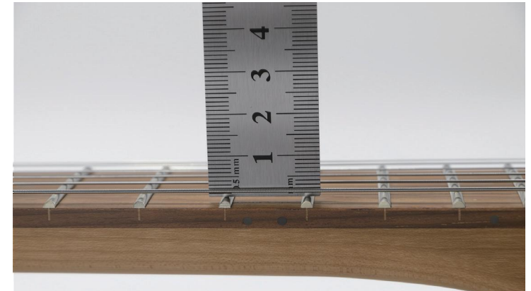
Treble side (1st string) at the 12th fret
